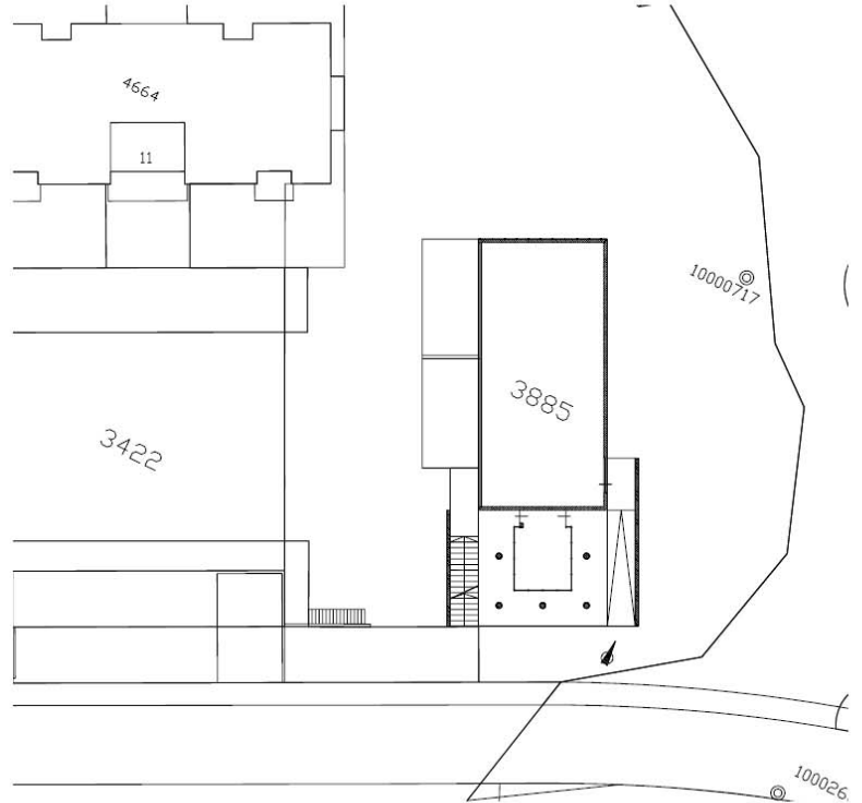
Situationsplan 1:500
